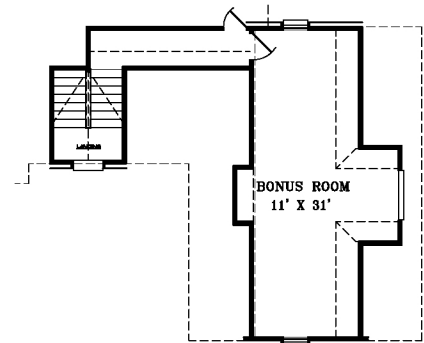
BONUS PLAN SECOND FLOOR
